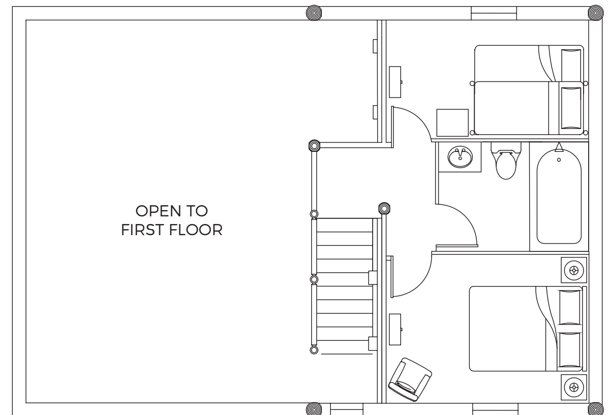
SECOND FLOOR
